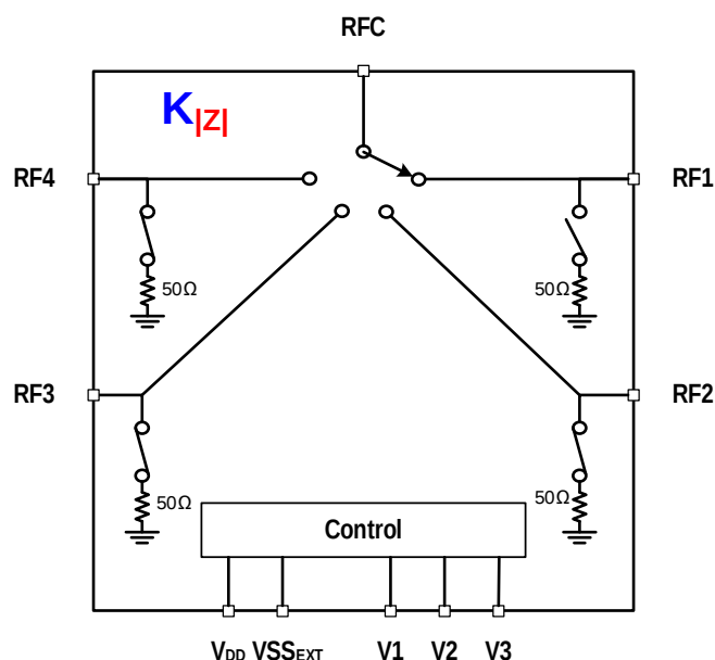
Figure 1. Block Diagram
