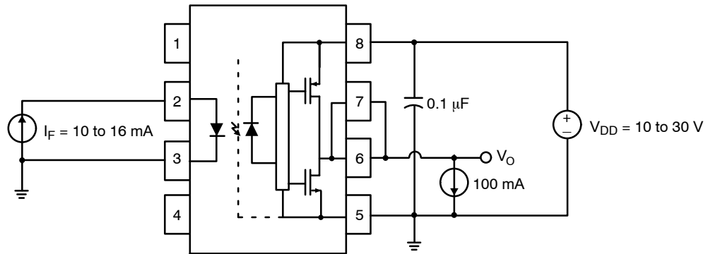
Figure 22. V_{OH} Test Circuit
