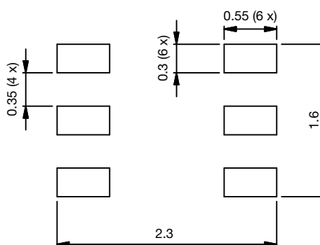
Recommended Footprint
