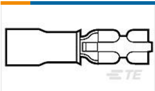
TE Part #640921-1 RECEPT,IDG FASTON 22-18 110
