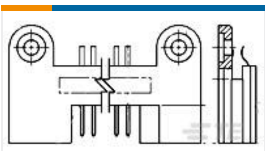
TE Part #530785-9 BOX PIN 80 POS 075 CL
