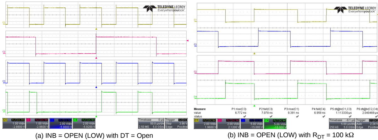
Figure 6. Experimental Waveforms of ANB Function with Dead-Time
