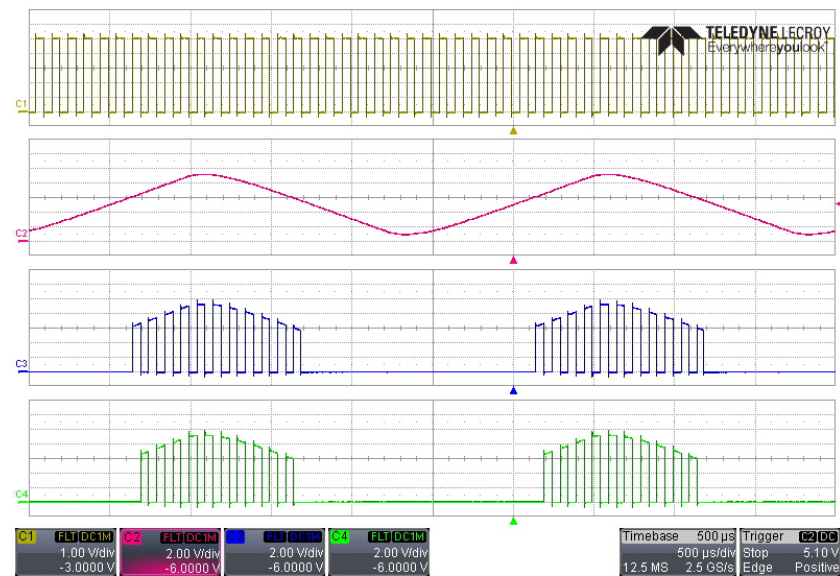
Figure 11. Experimental Waveforms of VCC Under-Voltage Lockout Protection
