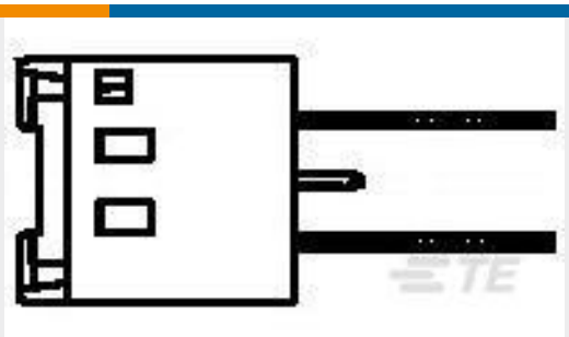
TE Part #1871845-3 GIC 2.5 ON TAPE HDR TIN VERSION 3P
