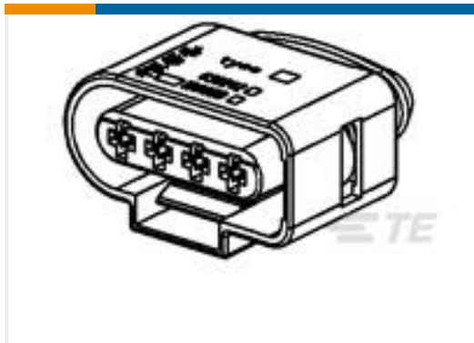
TE Part #638245-2 Receptacle Assembly, 4 position, Sealed,
