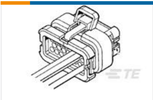
TE Part #776164-1 35POS,AMPSEAL,SOC HSG ASSY,SLD, COD 1
