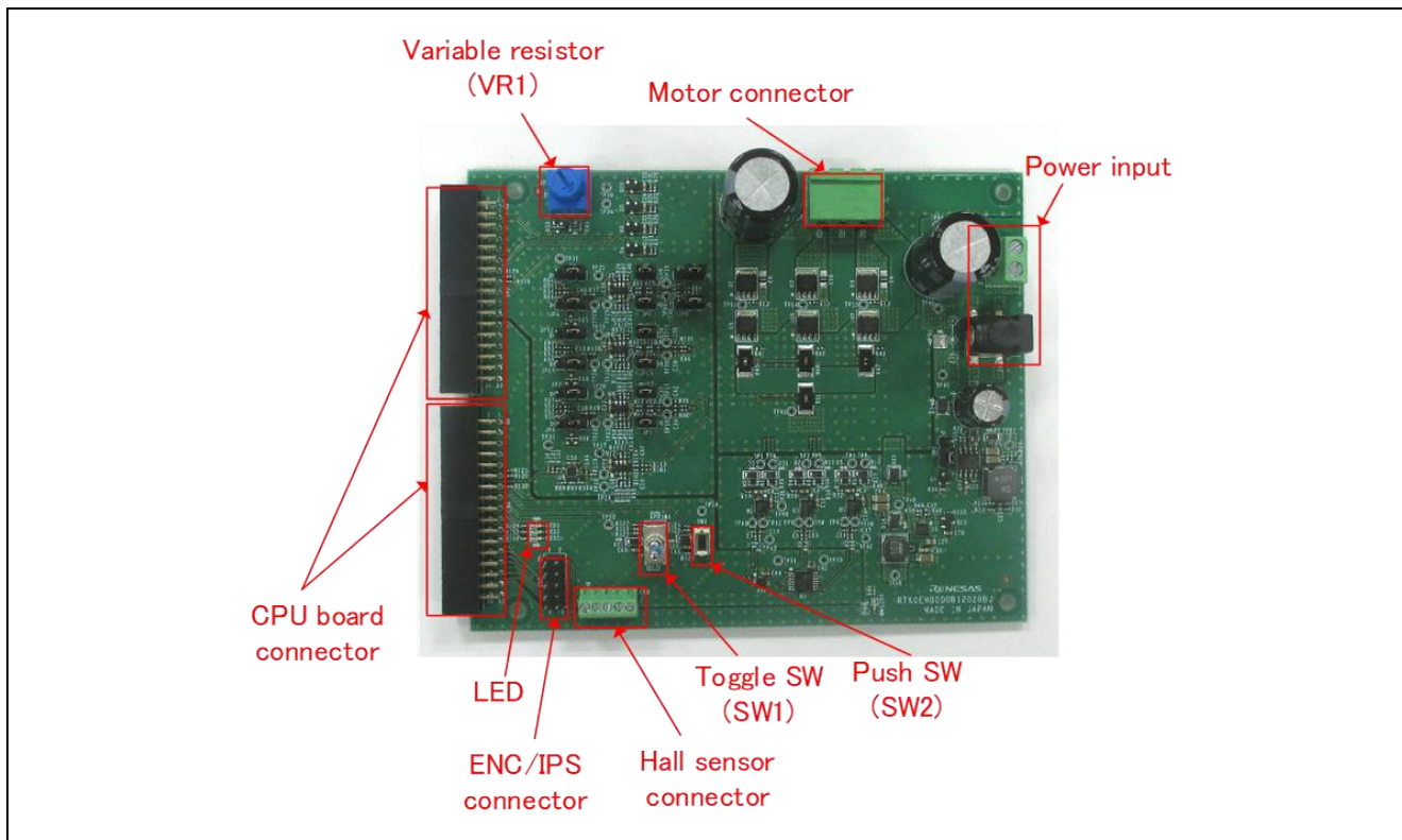
Figure 4-2 Inverter Board
