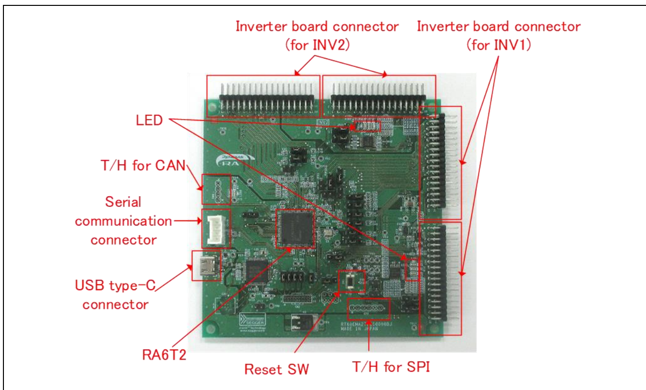
Figure 4-3 CPU Board
