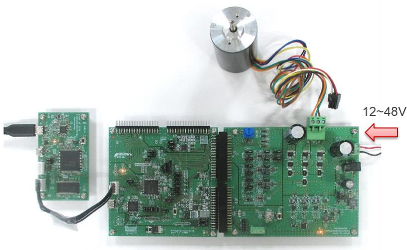
Figure 4-11 Power supply from terminal block
