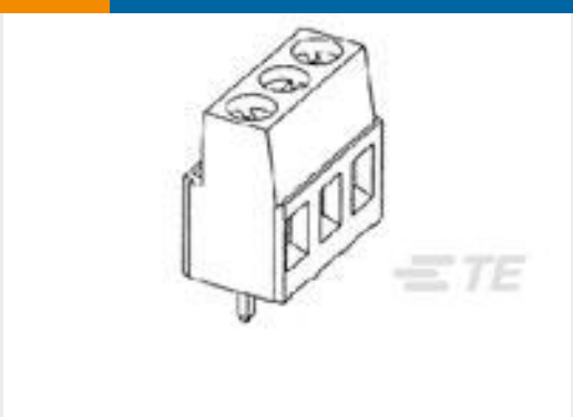
TE Part #796949-9 9 POS TERMI-BLOK PCB MOUNT
