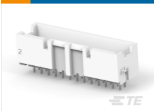
TE Part #2-2324245-6 ASSY,HDR,VERT,GWT,BOSSSED,DUAL ROW, EP2.5
