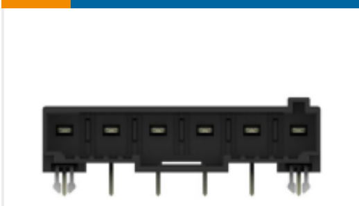
TE Part #1-2271457-6 D3950 HDR 6POS 1ROW X KEY
