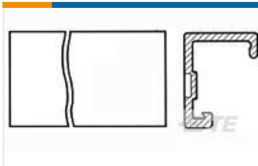
TE Part #640551-2 02P MTA156 COVER
