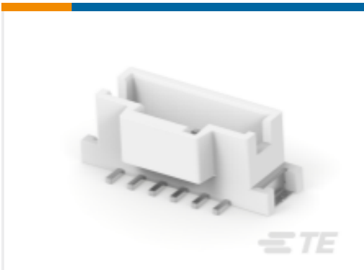
TE Part #1-2232829-6 SGI2.0 HEADER ASSEMBLY SMT 6P, KEY A,NTL
