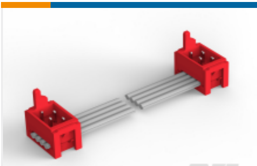
TE Part #2205066-1 MICRO-MATCH STD MOW TO MOW CABLE ASSY
