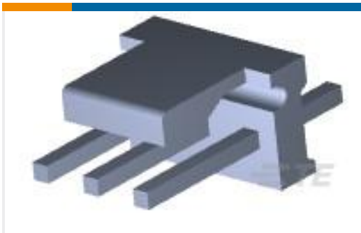
TE Part #644752-3 03P MTA156 HDR ASSY SQ STR F/L
