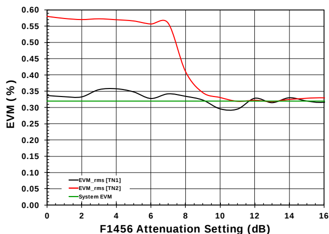
Figure 51. EVM (RMS) vs. Attn [2.65GHz]
