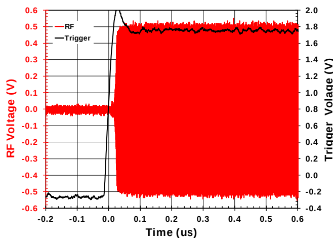
Figure 43. Switching Speed 31.5 to 0.0 dB
