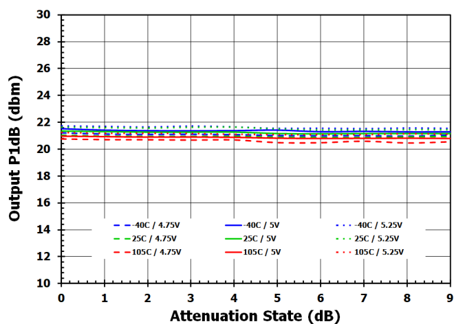
Figure 61. Output P1dB Vs. Attenuation [1.8GHz]
