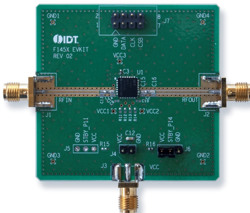
Figure 65. Top View
