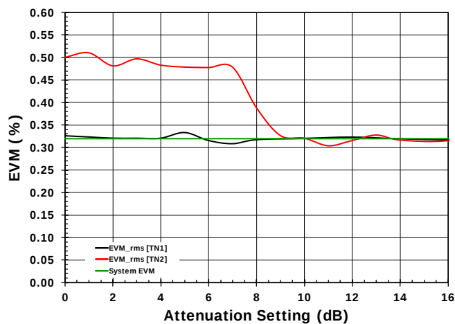
Figure 49. EVM (RMS) vs. Attn [2.5GHz]
