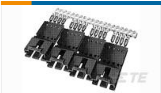
TE Part #103945-1 8X2 MTE SHRD PIN SR LATCH .100
