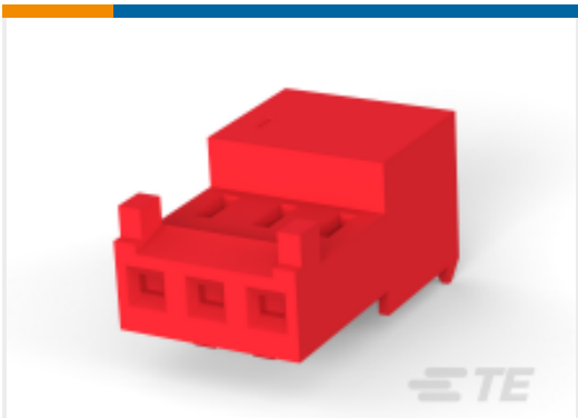
TE Part #3-643813-4 Nylon Tin Plated Receptacle: 2.54 mm, with Mating Alignment, MTA 100
