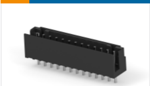
TE Part #292132-3 CT 2mm Post Header Asmby: Box V DIP
