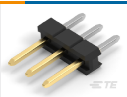
TE Part #2355177-3 3P,2MM,BRK HDR,SRVT,2.8,0.38AU,TB
