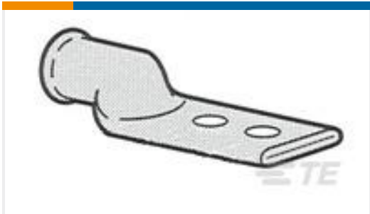
TE Part #53683-2 TERMINAL,AMPOWER 4/0 1/2
