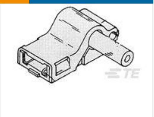
TE Part #1-480306-1 250 FASTON INSULATION POD.,REC., NATURAL
