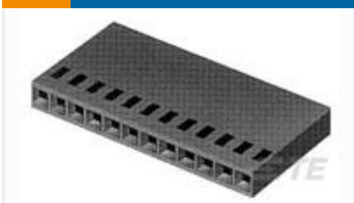
TE Part #2-87499-3 13 MODIV HSG SR MRKD .100CL
