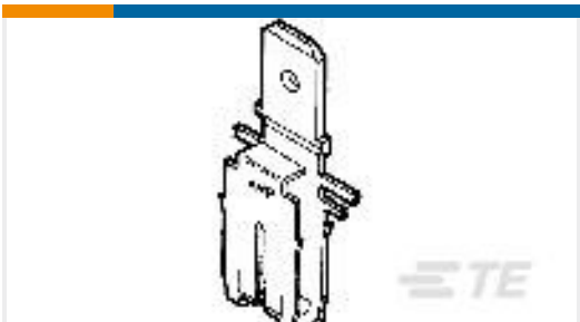
TE Part #63459-3 MAG-MATE 250 F-TAB 15-16 TPBR
