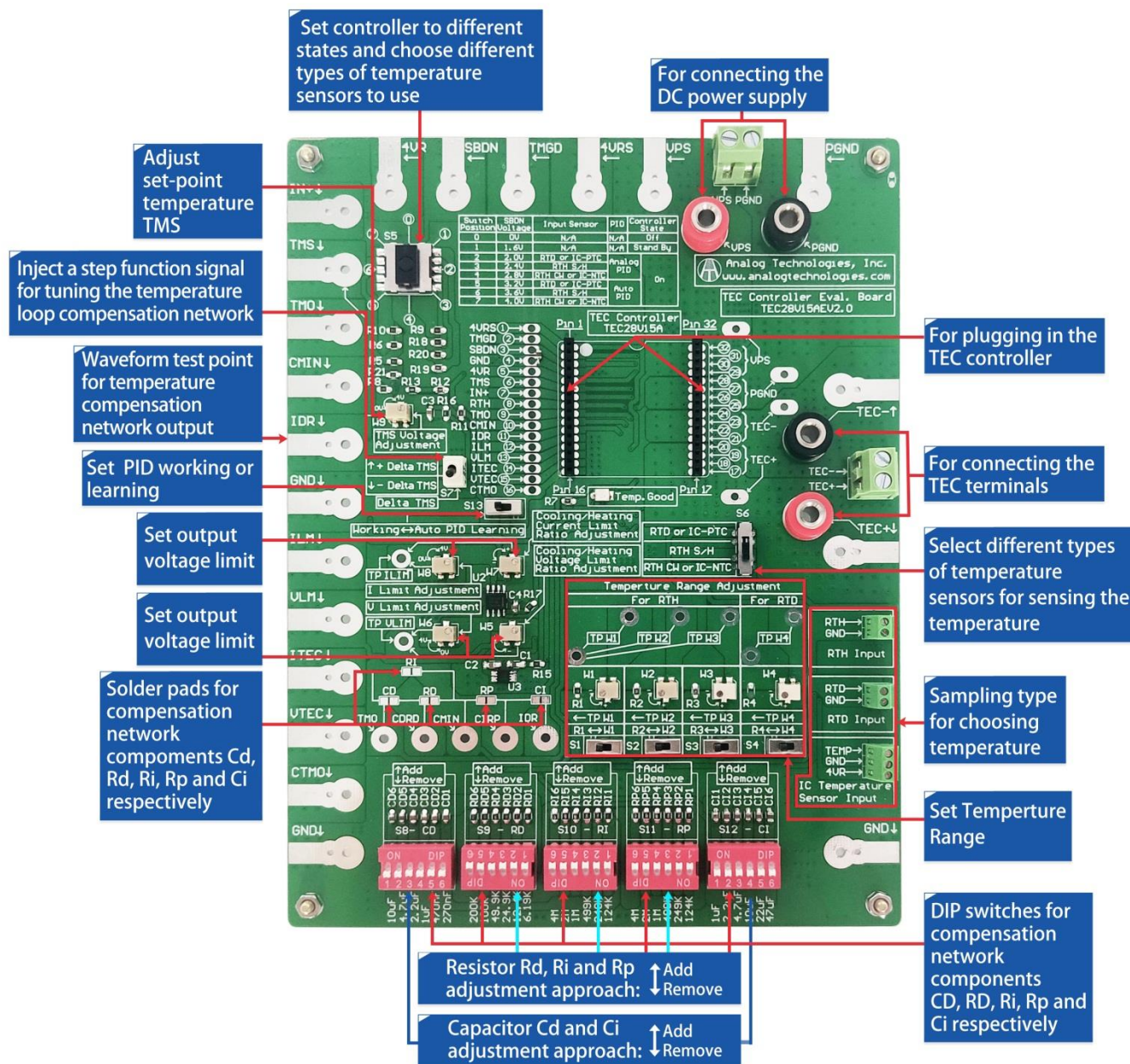
Figure 3. Board Description
