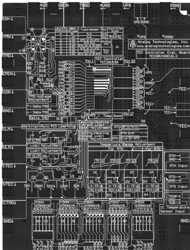
Figure 2. Top Silkscreen Layer with Other Top Layers
