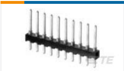
TE Part #87220-3 03 MODII HDR SRST UNSHRD .100
