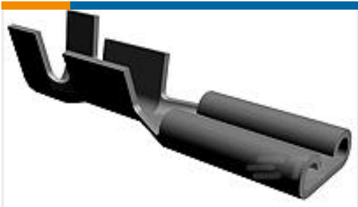
TE Part #61813-1 093 FASTON REC 26-22 AWG TPBR
