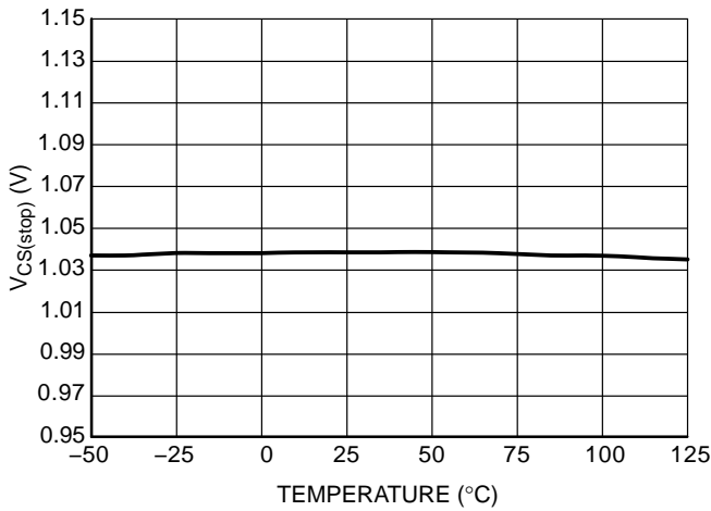
Figure 11. Threshold for Immediate Fault Protection Activation V CS(stop)
