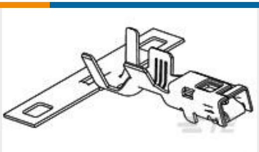
TE Part #1326032-3 2.8MM RECP,SEAL,18AWG
