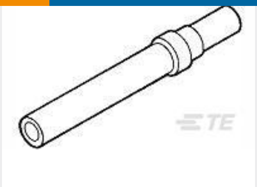
TE Part #1218267-1 CONT,CRIMP SKT,18AWG,109,SZ 20
