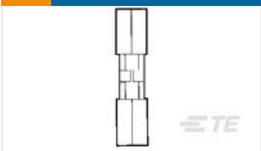
TE Part #324893 SPLICE,SOLIS BUTT STRAP 12-10
