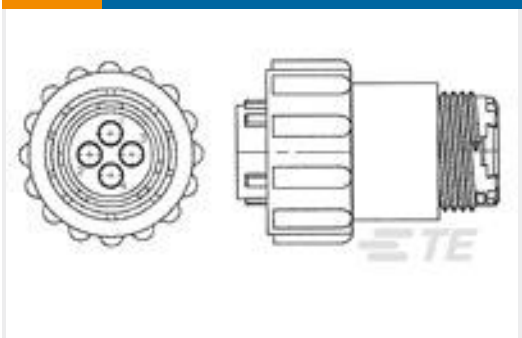
TE Part #788157-2 SLD CPC PLUG ASSY,13-9,STD SEX
