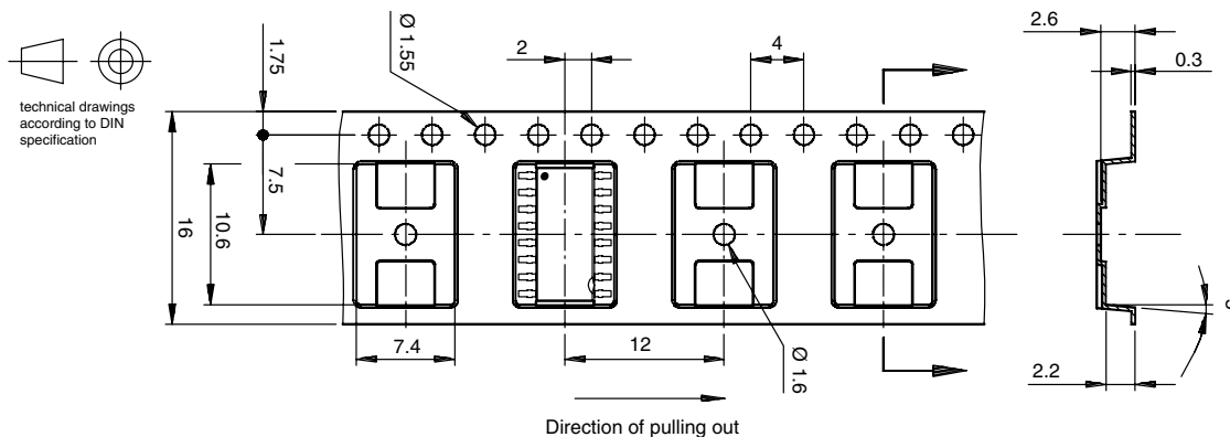
Fig. 16 - 2000 pcs/reel
