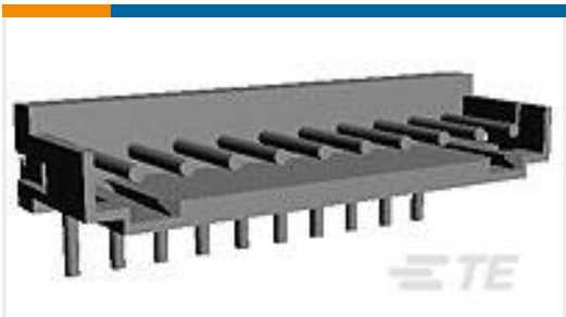
TE Part #292253-3 CT CONN MT HDR ASSY H 3P NAT
