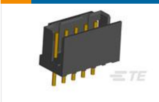
TE Part #292133-2 CT P/HDR ASSY BOX V 2P W/O KIN
