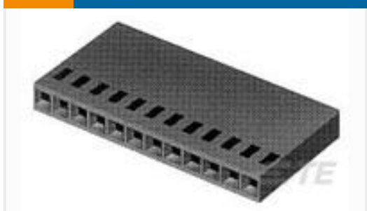
TE Part #5-87499-8 30 MODIV HSG COMP SR .100CL
