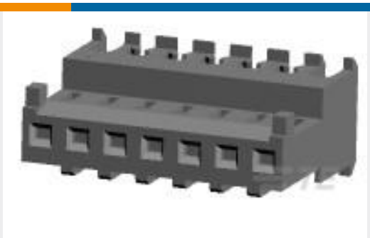
TE Part #3-644540-7 07P MTA100 CONN ASSY F/T POL
