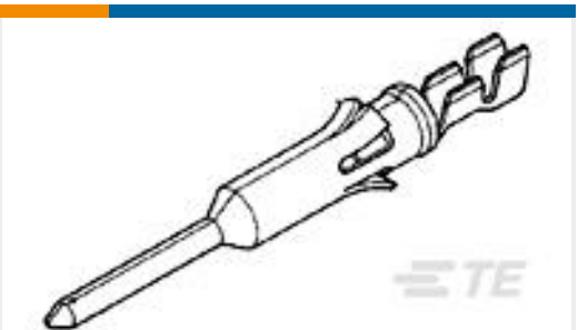
TE Part #66591-4 TYPE VI PIN,MULTI-MATE,L.P.
