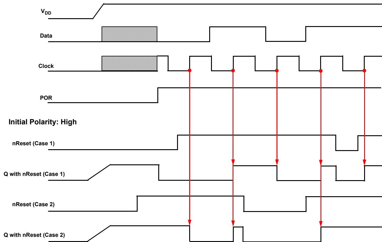
Figure 28. DFF Polarity Operations
