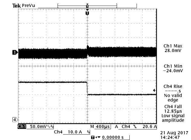
Figure 18. V_{in}=11V , V_o=1.8V , I_o=75\%-50\%I_o \text{ max} , di/dt=1A/us
