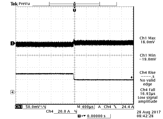
Figure 16. V_{in}=11V , V_o=1.0V , I_o=75\%-50\%I_o \text{ max} , di/dt=1A/us
