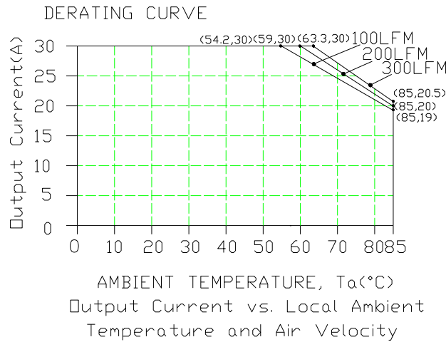
Figure 10. Test Condition: V_{out1} = 3.3V/30A ; V_{out2} = 3.3V/30A at V_{in}=11V@T_a=25^{\circ}C
