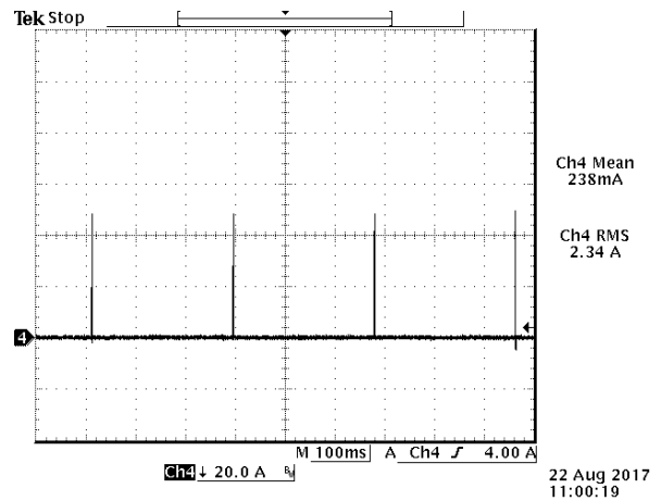
Figure 28. Vout2 Output current @ SCP, V_{in} = 11V , V_{out} = 2.5V , T_a = 25^\circ C
